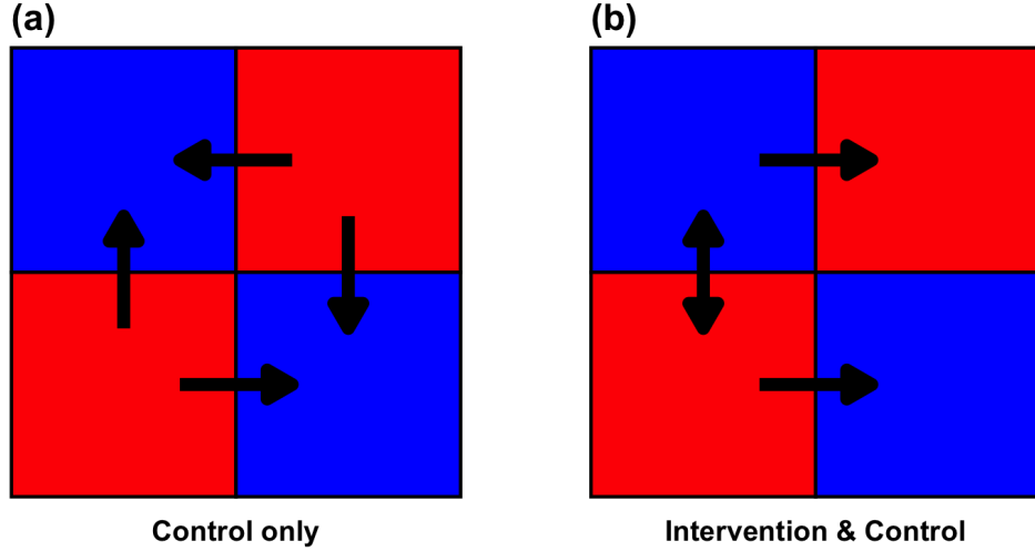
Figure 2: (a) Spillover application from intervention cells (red) to only control cells (blue) & (b) spillover application to intervention (red) and control cells (blue).
